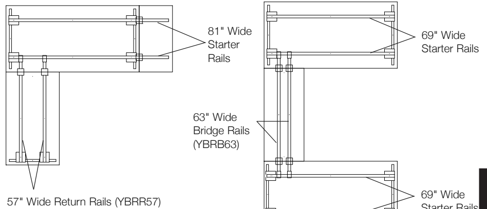
72" W, 24"D Desk with Extension Top and 54" Wide Return
