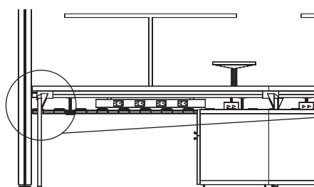
Elevation of conduit to Antenna Workspaces Single-Sided Basic Big Table
