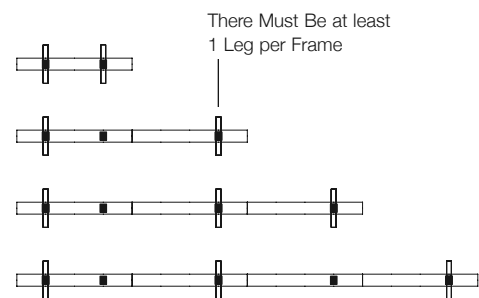
Straight Run Configurations using 48"W Frames
