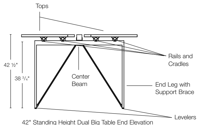
42" Standing Height Two Position Dual Big Table with End Legs and Support Braces
