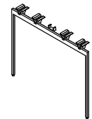
42" Standing Height End Leg Leg with Top: 42 1/2" Leg with Cradles: 41" Leg Weldmount: 39"
