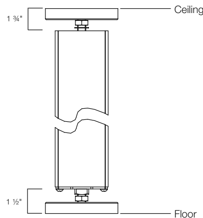
Ceiling/Floor Detail
