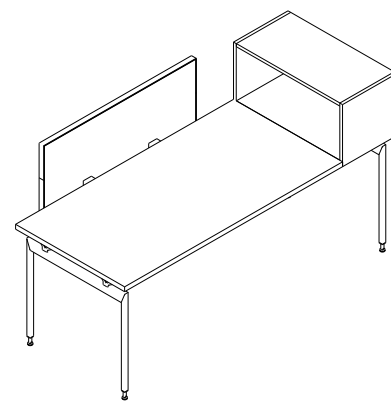
Desk with Adjustable Height End Legs and Suspended File
