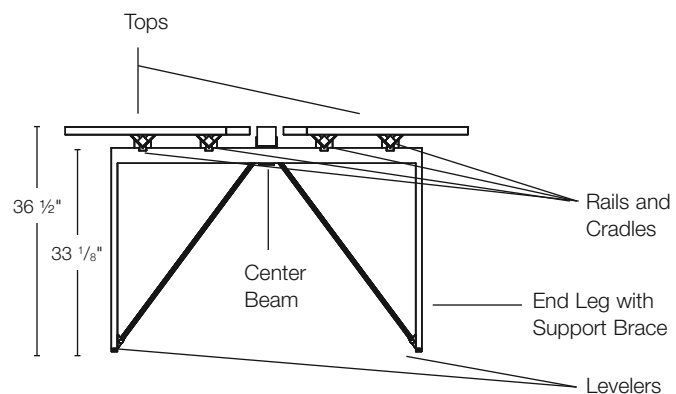
36" Standing Height Dual Big Table End Elevation
