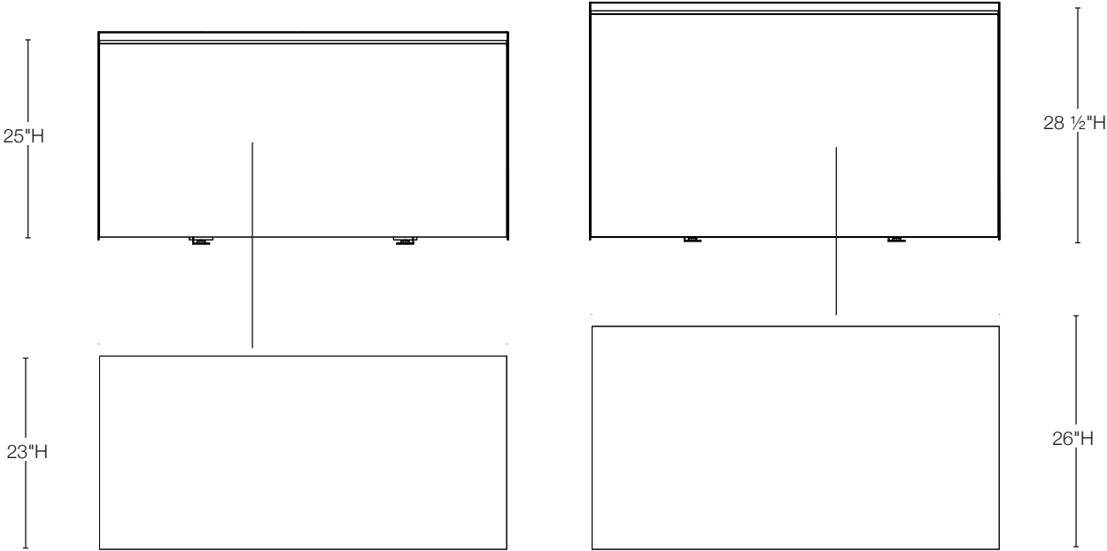
Paint/Laminate/Veneer Cover
