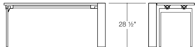
28 ½"H Fence Elevations
