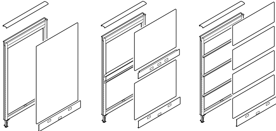
Monolithic Panel
