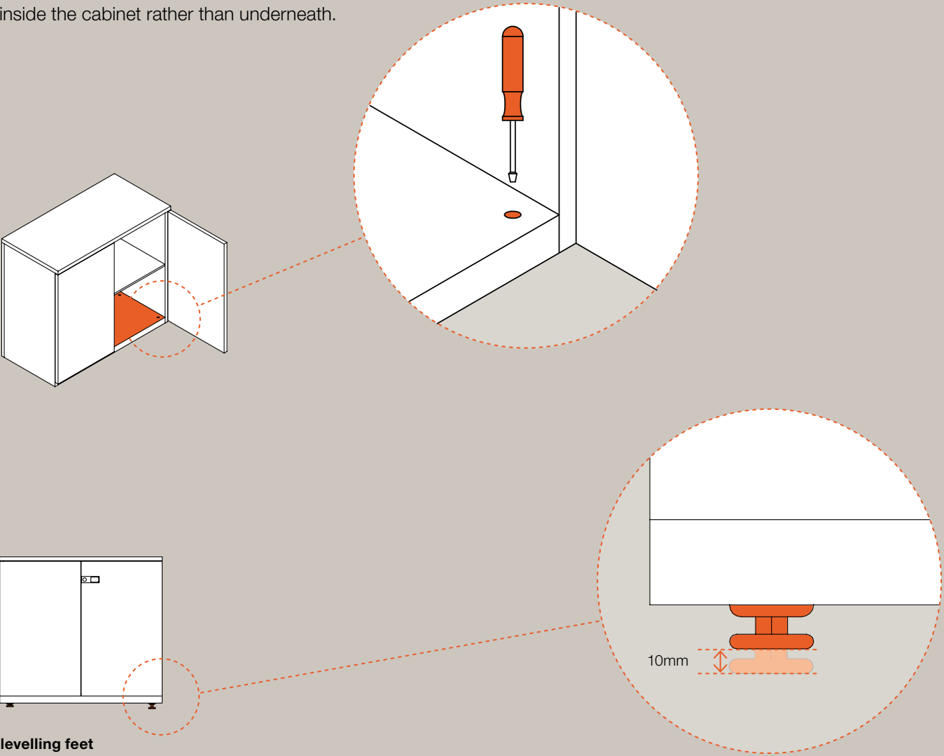
levelling feet 725 mm +/- 5mm, 720 +10mm, 730 -10mm
