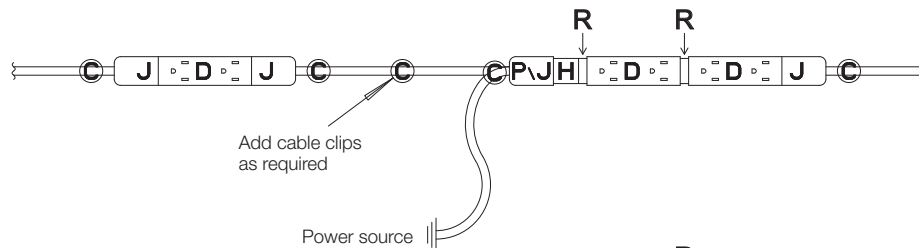
Split Power Entry Schematic (Option #1)
