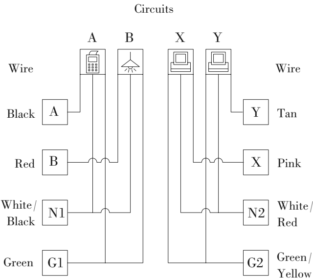
Wiring Diagram (2+2)
