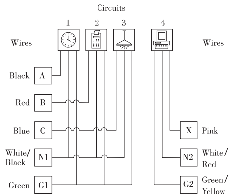
Wiring Diagram (3+1)
