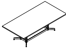
Rectangular W: 69.25, 79.25" D: 34" H: 29"
