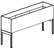
Freestanding Planter W: 30, 36, 42, 48, 54, 60, 66, 72" D: 15" H: 31"
