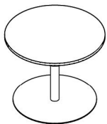
Column Base Table Round Top W: 36, 42" D: 36, 42" Fixed Height: 28.375" Height-Adjustable: 28-43"
