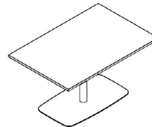
Column Base Table Rectangle Top W: 48, 54" D: 30, 36" Fixed Height: 28.375" Height-Adjustable: 28-43"
