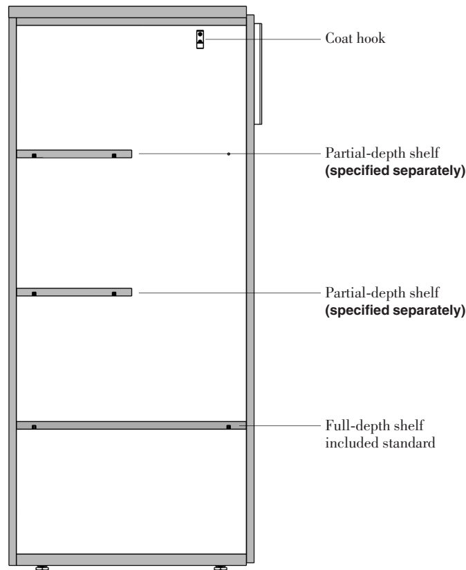
Locker cross-section
